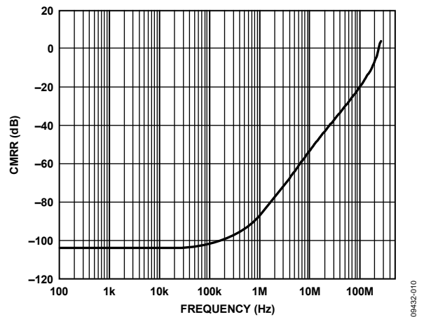
Figure 16. CMRR vs. Frequency ( G = 0.8 )
