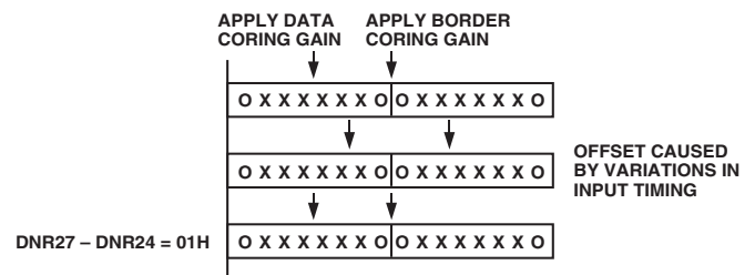
Figure 48. DNR Block Offset Control
