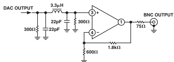
Figure 56. Example for Output Filter for PS, 8x Oversampling
