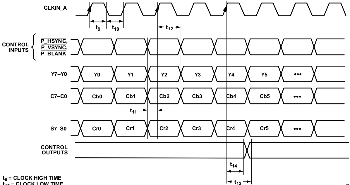
Figure 4. HD Only 4:4:4 Input Mode [Input Mode 010]; PS Only 4:4:4 Input Mode [Input Mode 001]
