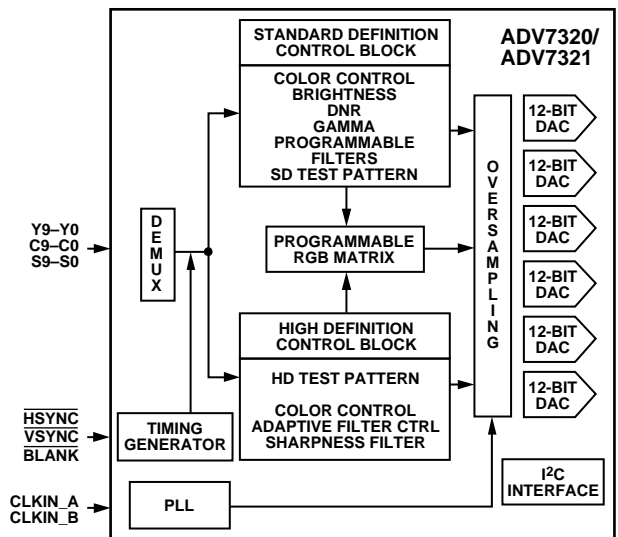
Figure 1. Simplified Functional Block Diagram
