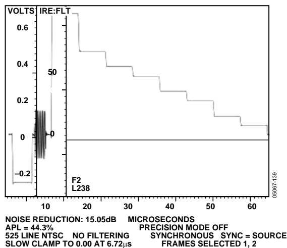
Figure 139. NTSC Luma
