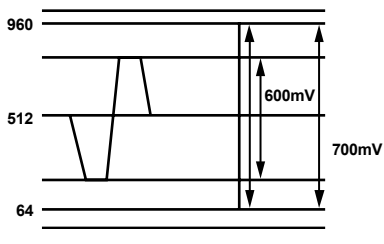
Figure 122. EIA-770.3 Standard Output Signals (1080i/720p)
