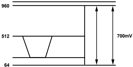
Figure 120. EIA-770.2 Standard Output Signals (525p/625p)
