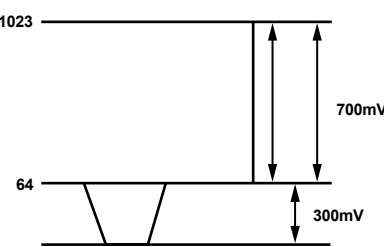
Figure 123. Output Levels for Full Input Selection
