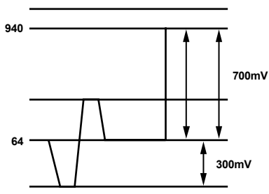
EIA-770.3, STANDARD FOR Pr/Pb OUTPUT VOLTAGE
