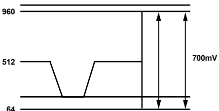
EIA-770.1, STANDARD FOR Pr/Pb OUTPUT VOLTAGE
