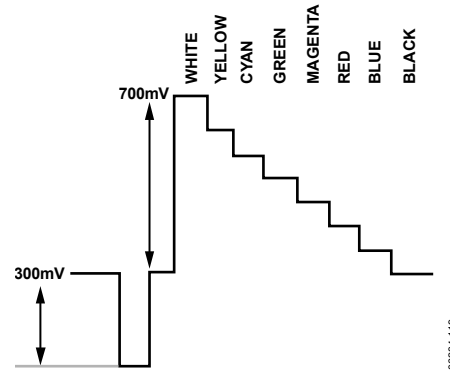
Figure 119. Y Levels—PAL
