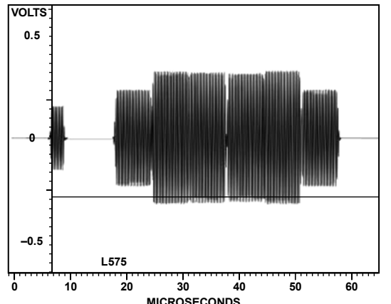
Figure 135. PAL Chroma
