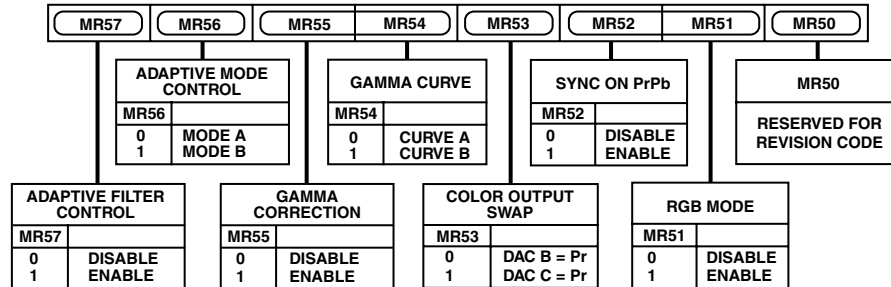
Figure 25. Mode Register 5
