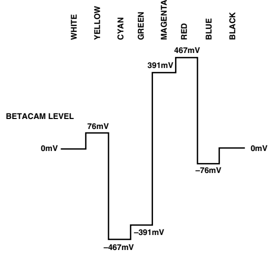
Figure 125. NTSC 100% Color Bars with Pedestal V
