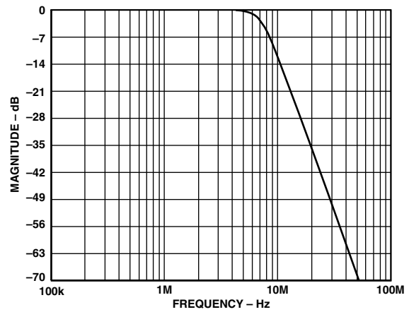
Figure 103. Output Filter Plot for 4× Oversampling Filter
