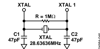
Figure 43. Crystal Circuit
