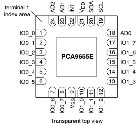
Figure 4. QFN24
