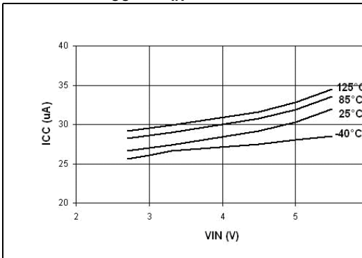
Figure 17. I_{CC} vs V_{IN} (enabled)
