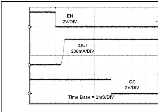
Figure 13. OC protection at V_{OUT} = 3.0\text{ V}
