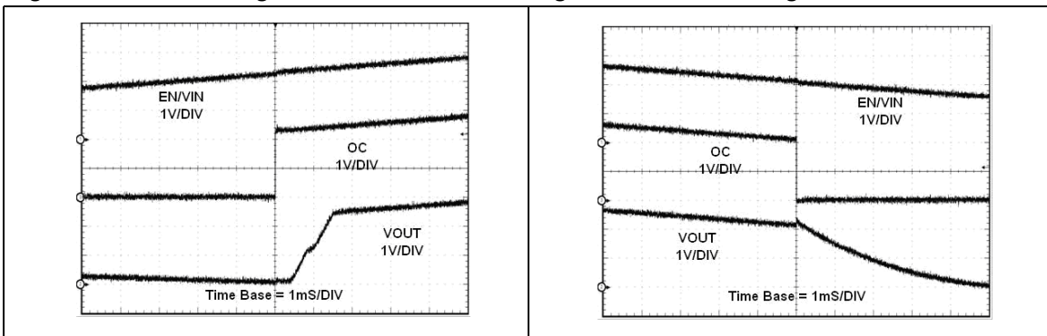
Figure 36. UVLO rising
