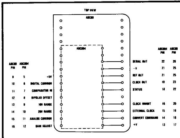
FIGURE 4. Adapting an ADC80 Layout for ADC804.
