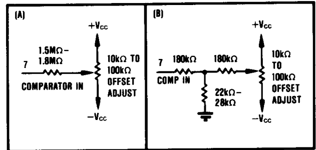
FIGURE 5. Two Methods of Connecting Optional Offset Adjust.
