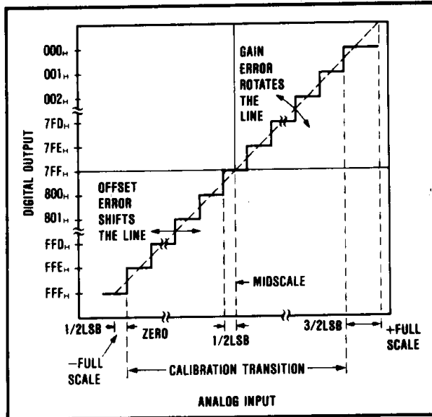
FIGURE 1. ADC804 Transfer Characteristic Terminology.
