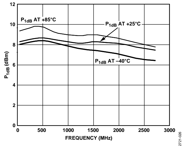
Figure 26. P_{1dB} vs. Frequency, V_S = 5\text{ V}, T_A = -40^\circ\text{C}, +25^\circ\text{C}, \text{ and } +85^\circ\text{C}
