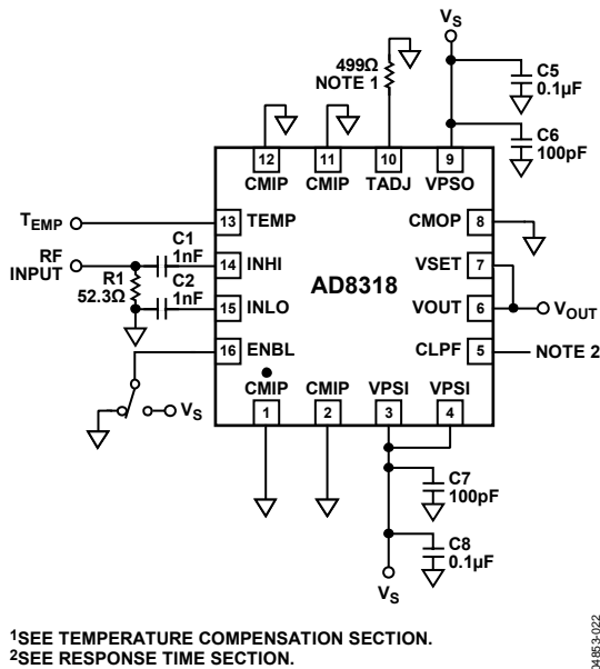
Figure 23. Basic Connections
