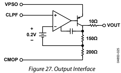
Figure 27. Output Interface
