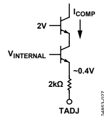
Figure 29. TADJ Interface
