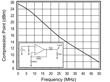
-1dBm Compression to Load
