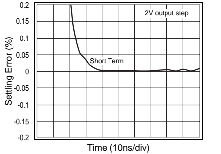
Short Term Settling Time
