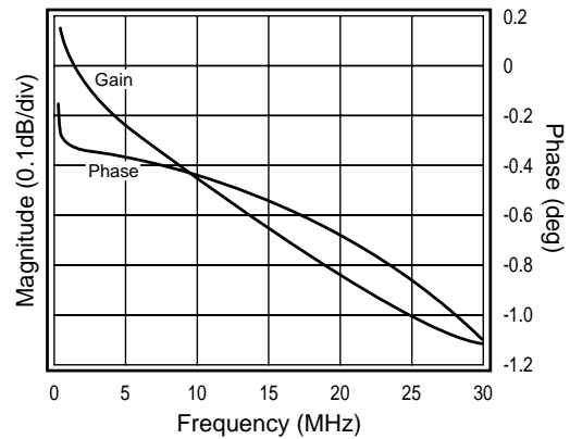
Gain Flatness & Linear Phase
