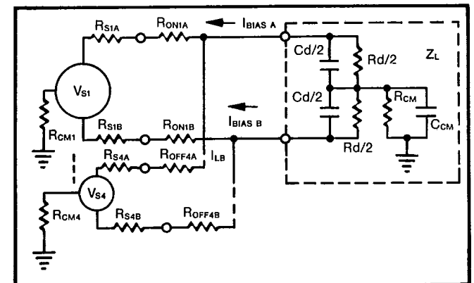
FIGURE 2. HI-509A DC Accuracy Equivalent Circuit.
