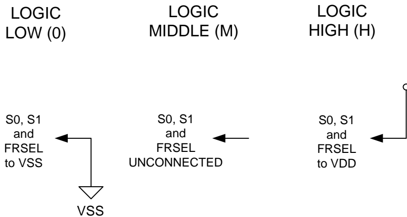
Figure 1. 3-Level Logic
