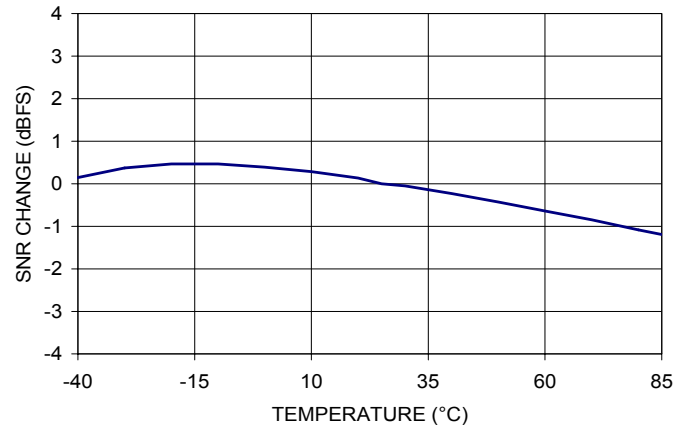
Figure 25. SNR Performance vs. Temperature after 25°C Calibration
