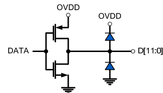
Figure 48. CMOS Outputs
