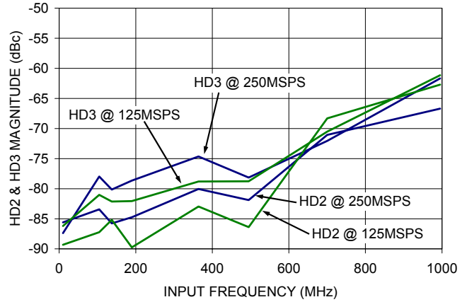
Figure 6. HD2 & HD3 vs. f IN
