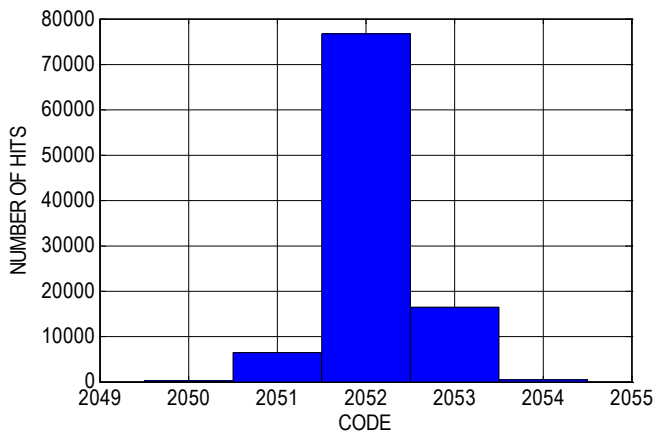
Figure 15. Noise Histogram
