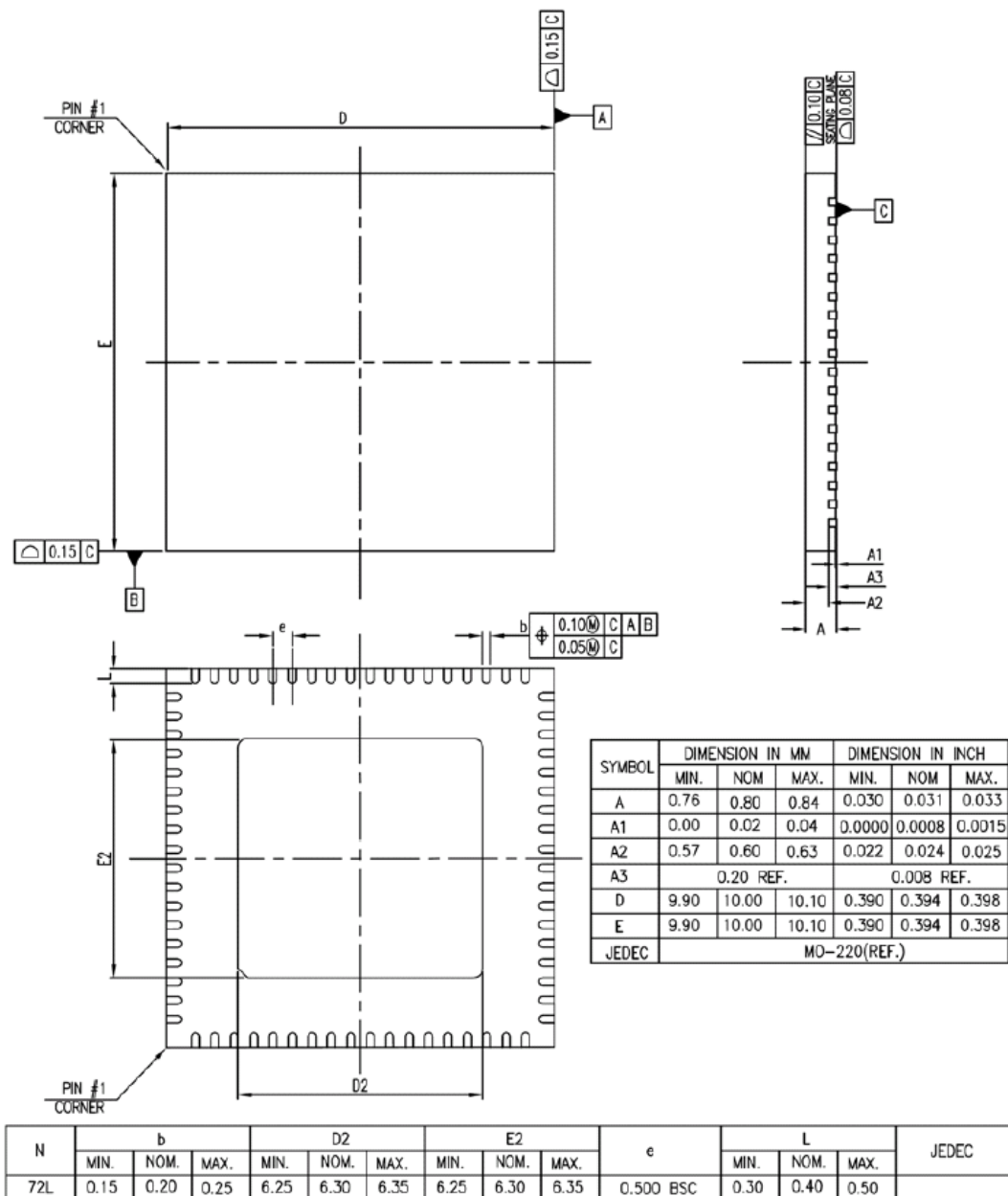
Figure 50. 72QFN Dimensions
