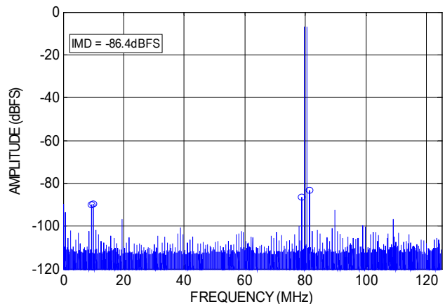
Figure 22. Two-Tone Spectrum @ 170 MHz
