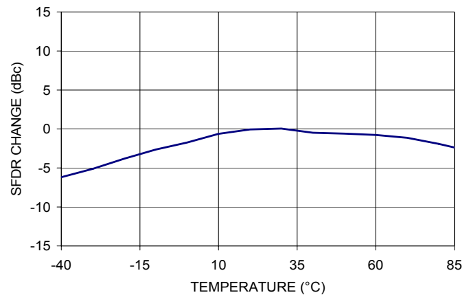
Figure 26. SFDR Performance vs. Temperature after 25°C Calibration
