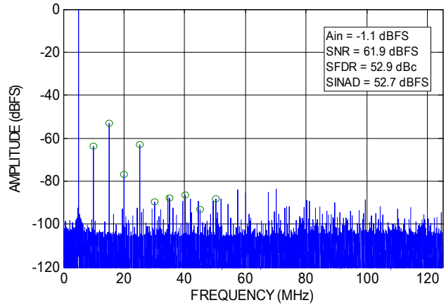
Figure 20. Single-Tone Spectrum @ 995 MHz
