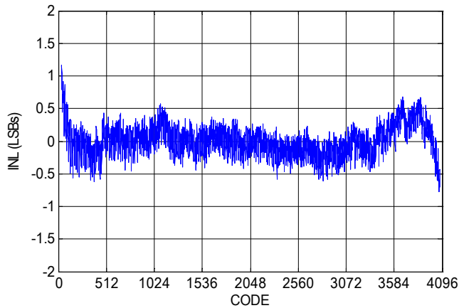
Figure 13. Integral Nonlinearity
