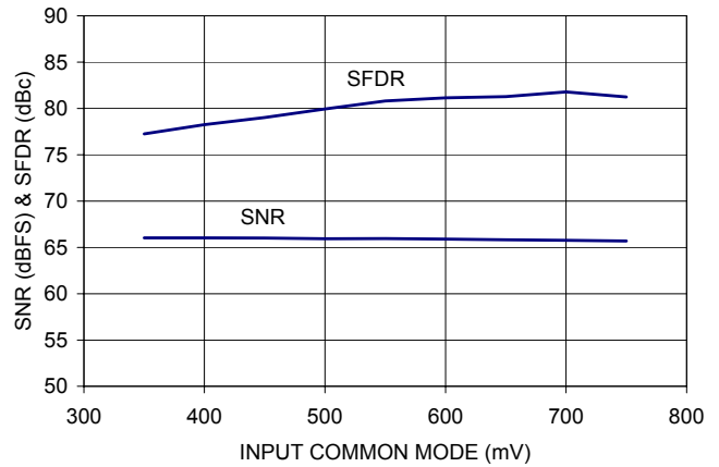
Figure 14. SNR & SFDR vs. VCM
