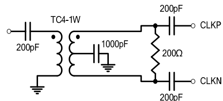
Figure 31. Recommended Clock drive
