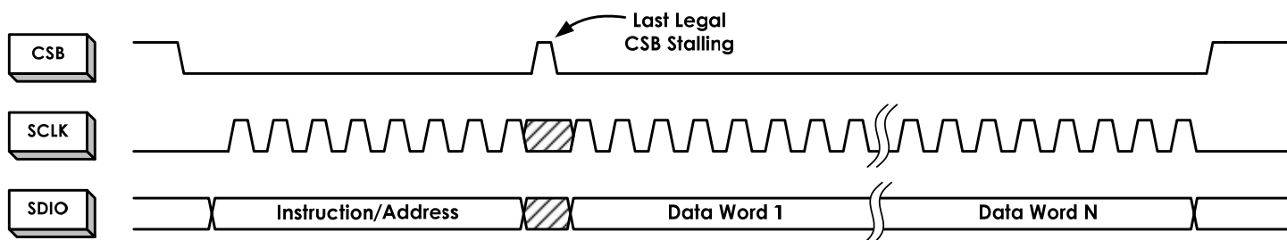
Figure 49. N-Byte Transfer
