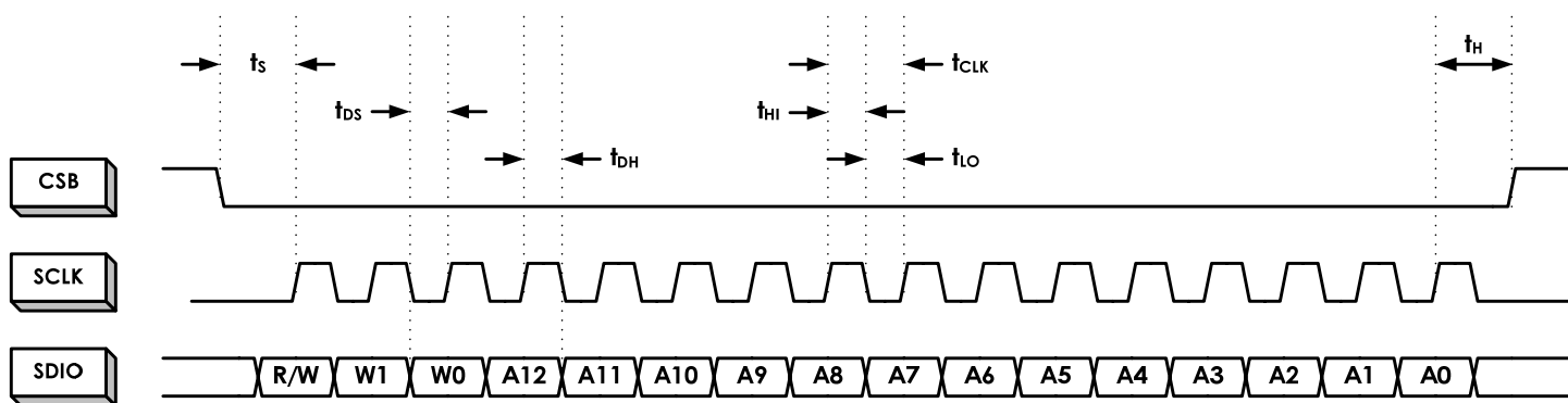
Figure 37. Instruction/Address Phase
