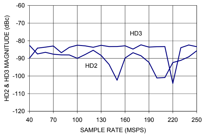
Figure 10. HD2 & HD3 vs. f SAMPLE
