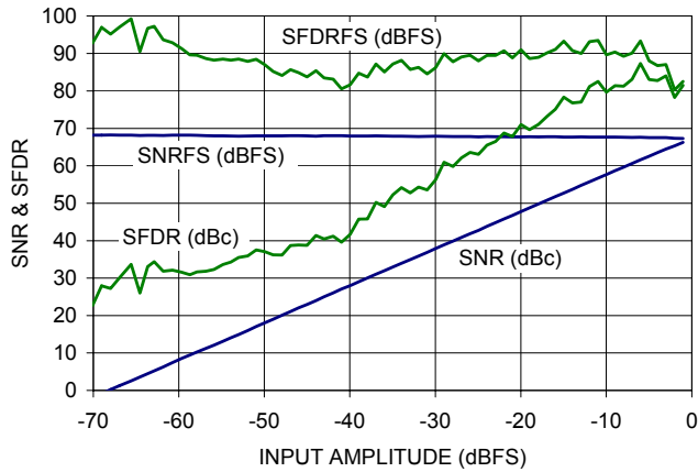
Figure 7. SNR & SFDR vs. A IN
