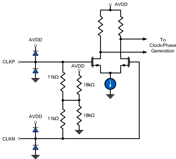
Figure 44. Clock Inputs
