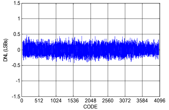
Figure 12. Differential Nonlinearity
