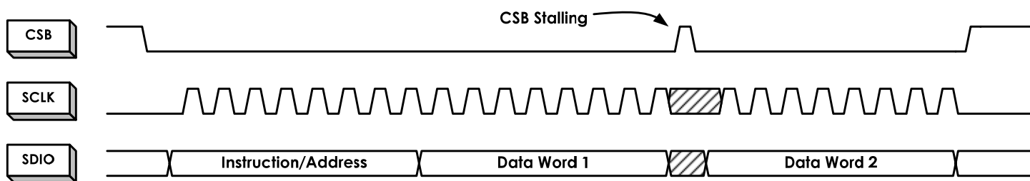
Figure 38. 2-Byte Transfer
