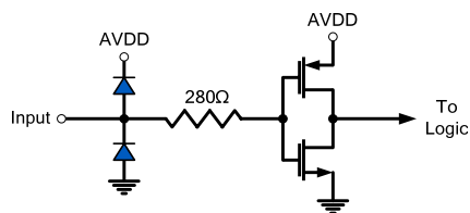
Figure 46. Digital Inputs
