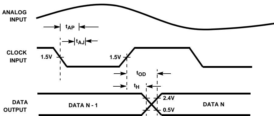
FIGURE 1. HI5766 INTERNAL CIRCUIT TIMING
