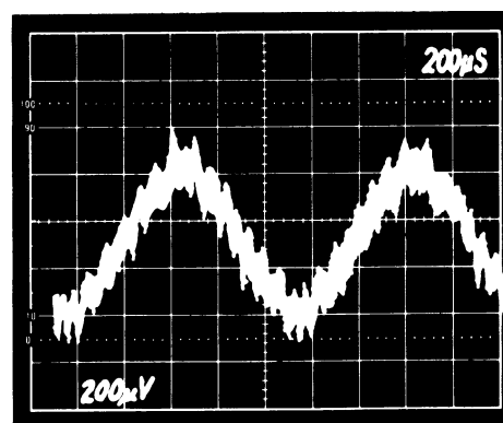
Figure 6. Midscale Differential Linearity
