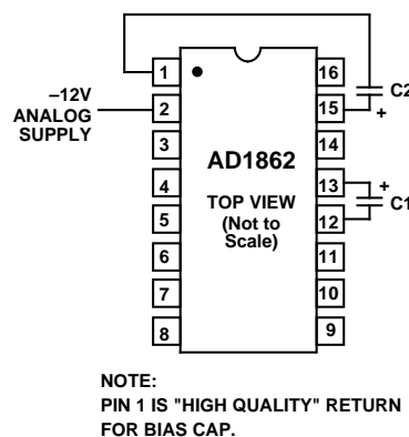
Figure 8. Noise Reduction Capacitors
