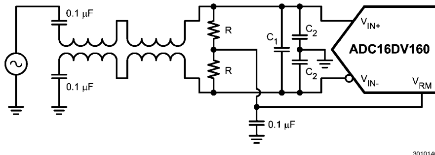
FIGURE 6. Transformer Drive Circuit for High Input Frequency
