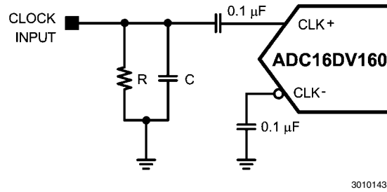
FIGURE 11. Singled-Ended 1.8V Clocking, Capacitive AC Coupled
