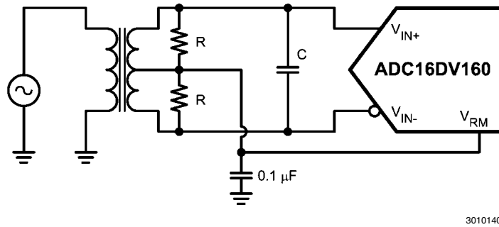
FIGURE 5. Transformer Drive Circuit for Low Input Frequency
