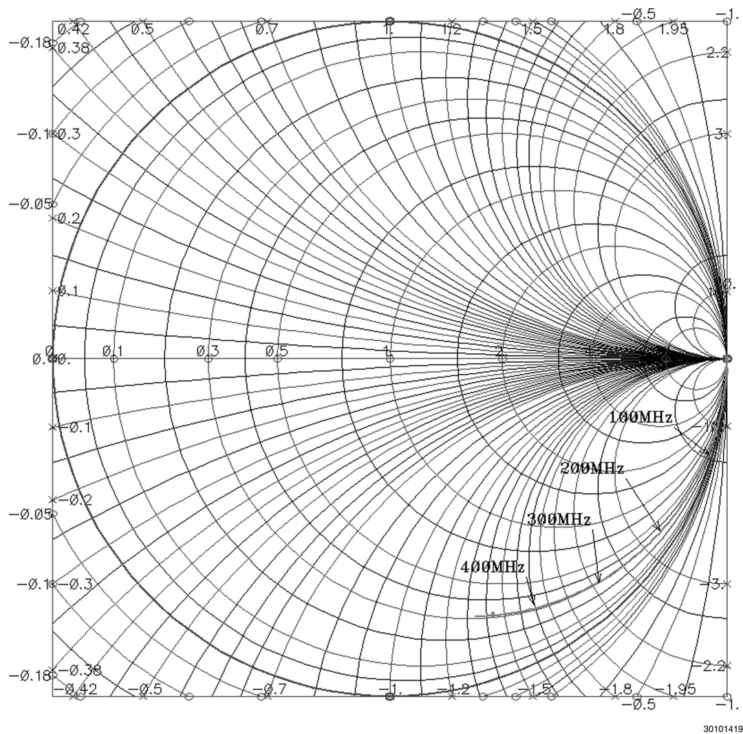
FIGURE 8. Simulated ADC16DV160 Input S11
