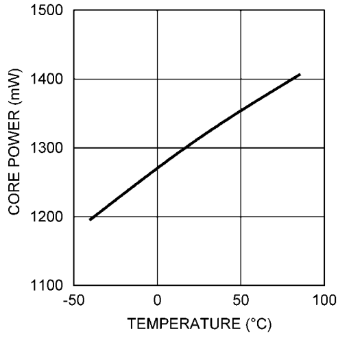
Core Power vs. Temperature (Excludes I_{DR} )
