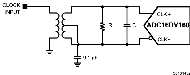
FIGURE 10. Differential Clocking, Transformer Coupled
