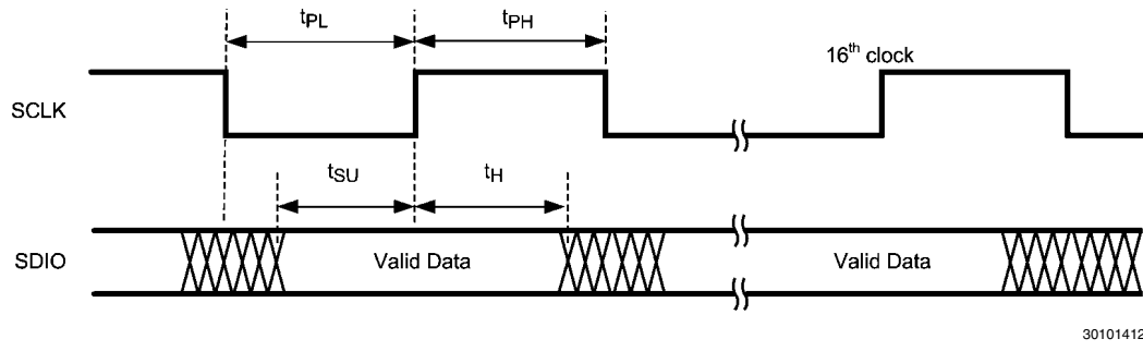
FIGURE 2. SPI Write Timing
