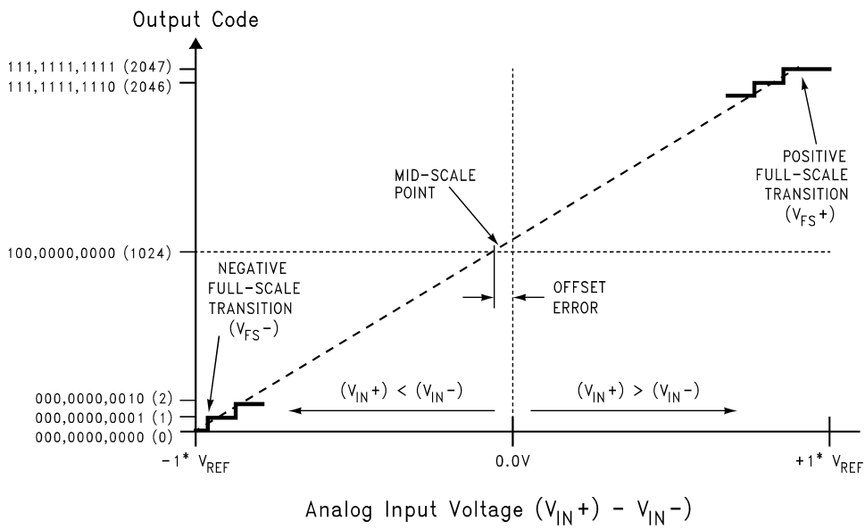
FIGURE 1. Transfer Characteristic
