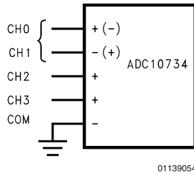
FIGURE 13. Analog Input Multiplexer Options
