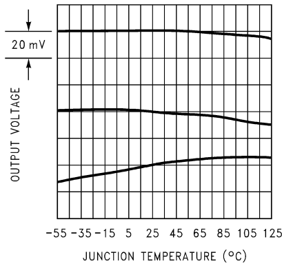
Output Drift vs. Temperature (3 Typical Parts)
