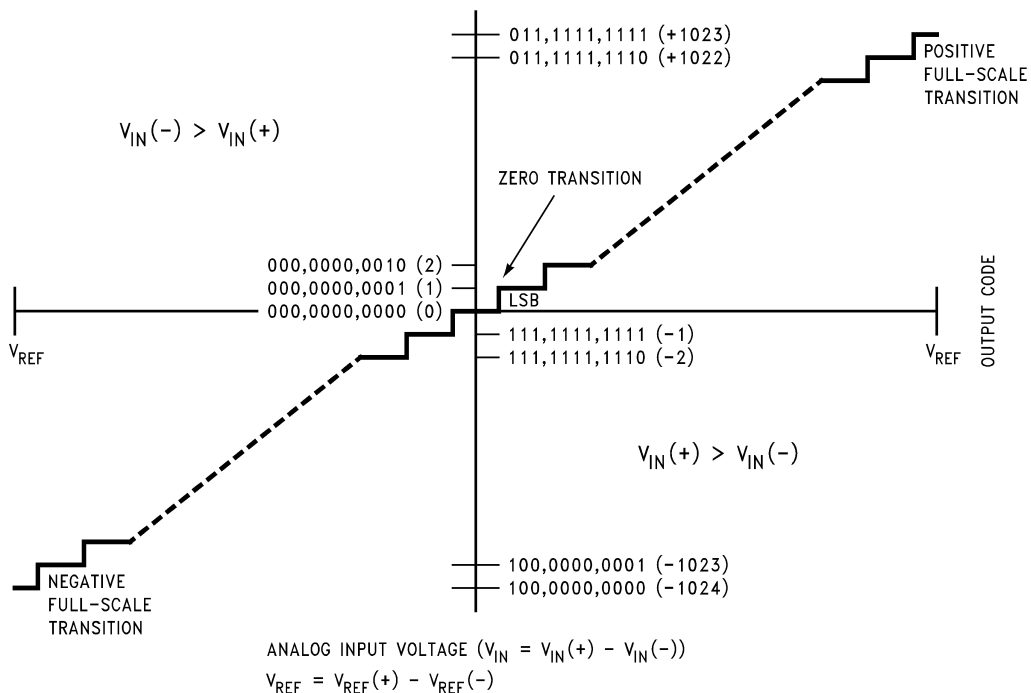
FIGURE 1. Transfer Characteristic
