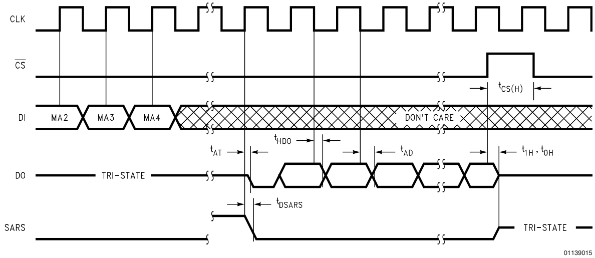
FIGURE 4. DO Timing
