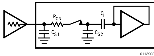
FIGURE 16. Analog Input Model
