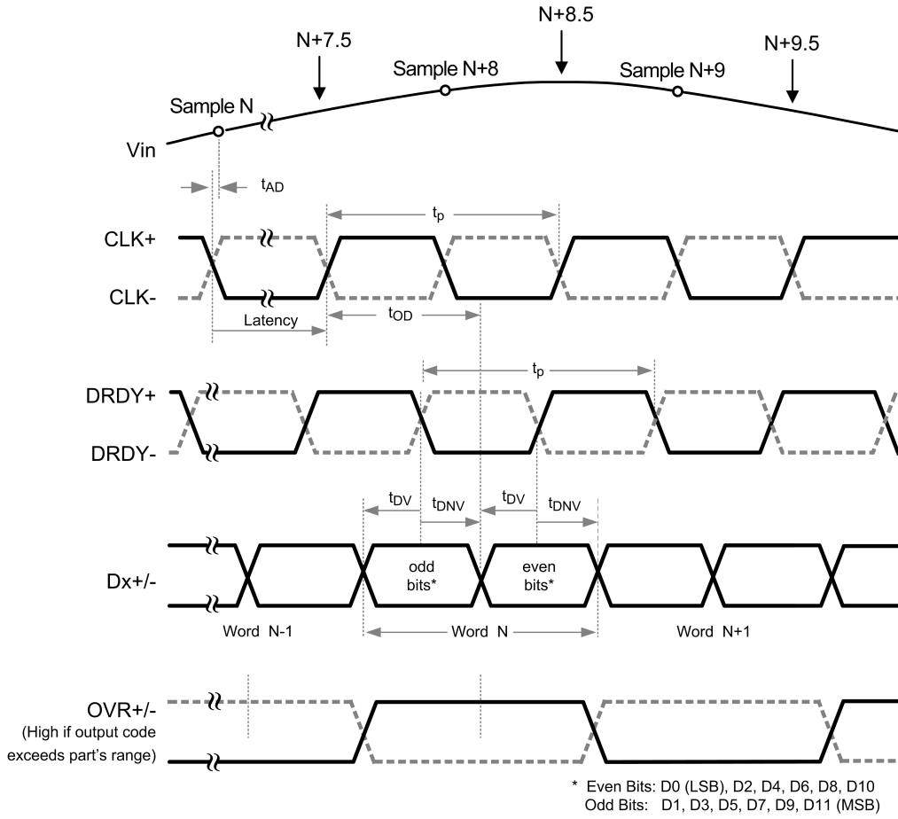
Output Timing
