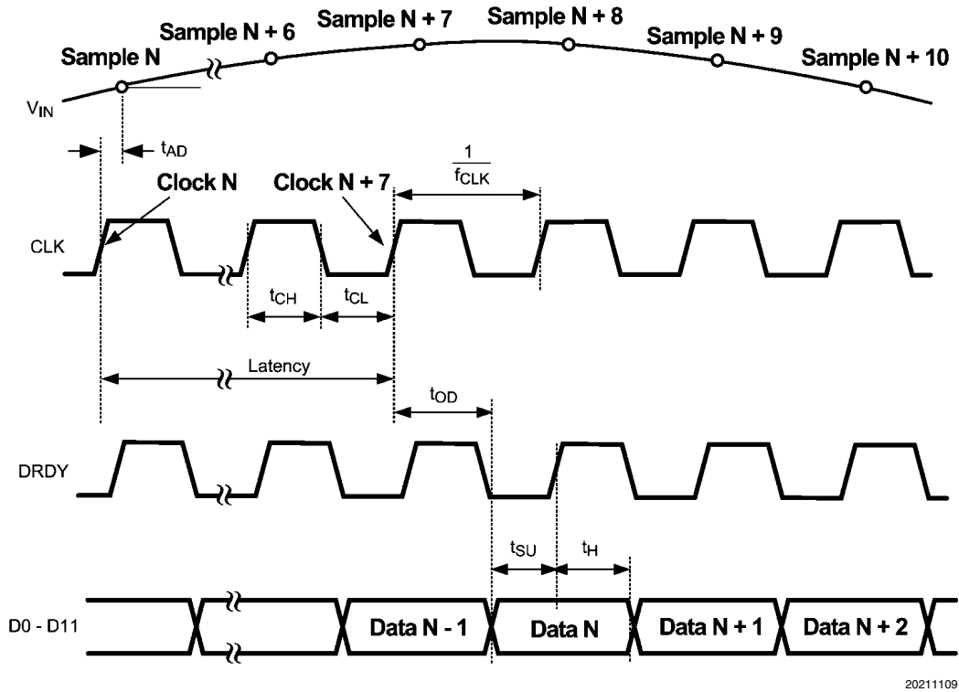
FIGURE 1. Output Timing
