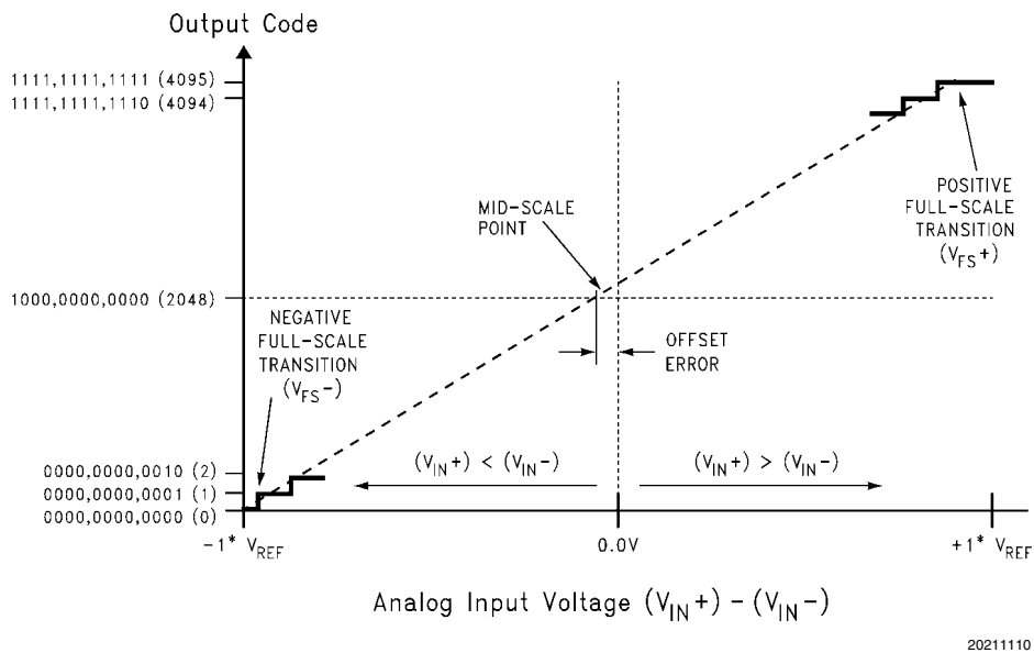
FIGURE 2. Transfer Characteristic
