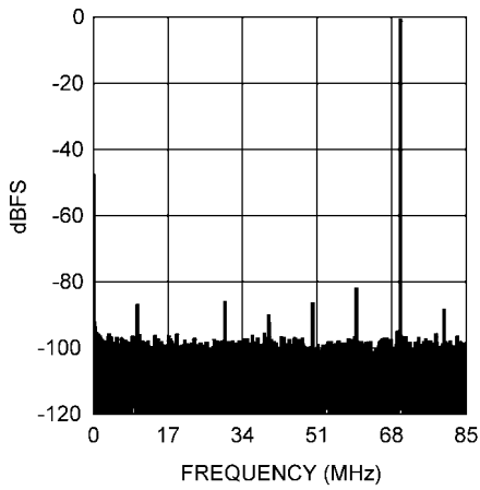
Spectral Response @ 70 MHz Input
