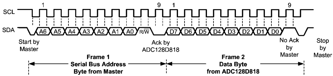
FIGURE 8. Serial Bus Interface Read Example 1 - Single Byte Read with Preset Internal Address Register.
