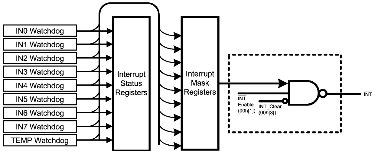
FIGURE 13. Interrupt Structure
