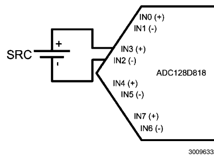
FIGURE 3. Pseudo-Differential Configuration
