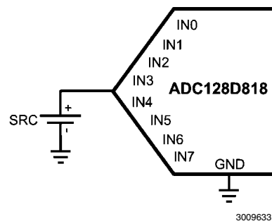
FIGURE 2. Single-Ended Configuration
