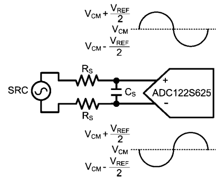
FIGURE 7. Differential Input
