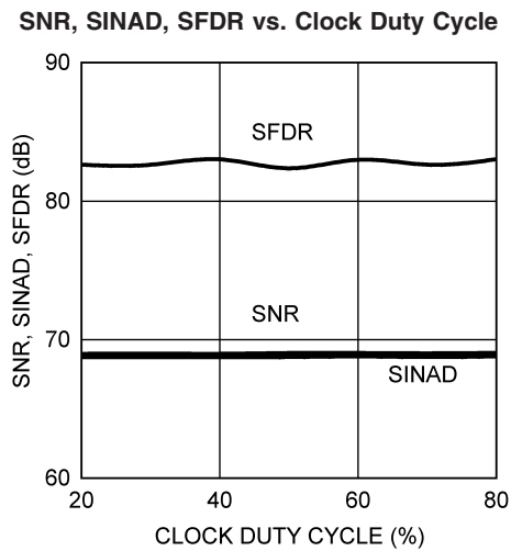
SNR, SINAD, SFDR vs. Clock Duty Cycle (DCS=OFF)
