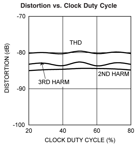
Distortion vs. Clock Duty Cycle (DCS=OFF)
