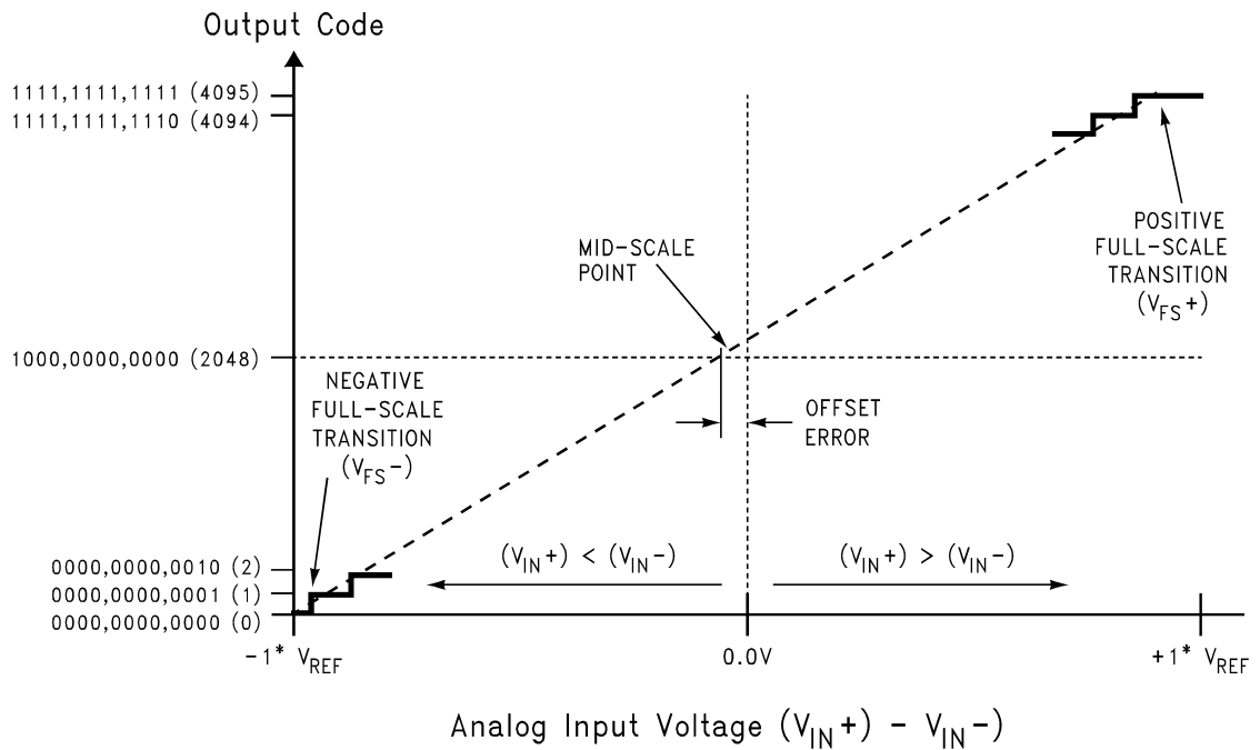
FIGURE 1. Transfer Characteristic
