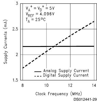
Supply Current vs Clock Frequency
