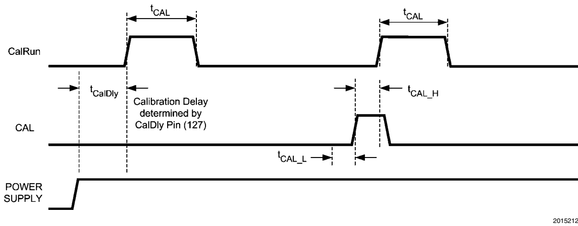
FIGURE 9. Self Calibration and On-Command Calibration Timing
