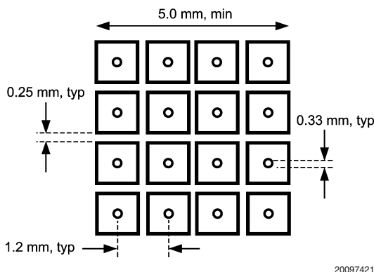
FIGURE 18. Recommended Package Land Pattern
