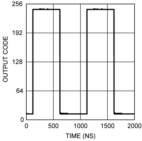
STEP RESPONSE
