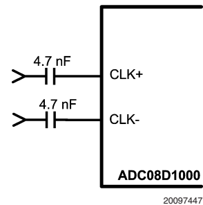
FIGURE 14. Differential (LVDS) Input Clock Connection
