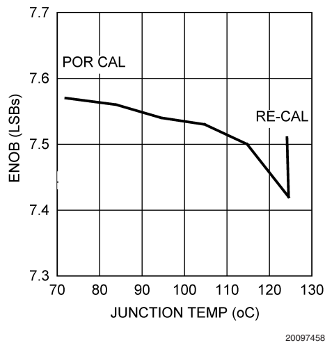
FIGURE 16. ENOB vs. Junction Temperature, 249MHz input
