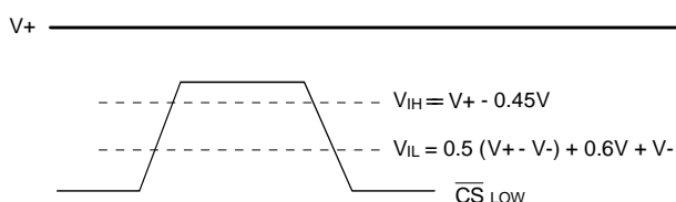
Figure 9. \overline{CS} and SCLK Digital Input Levels.
