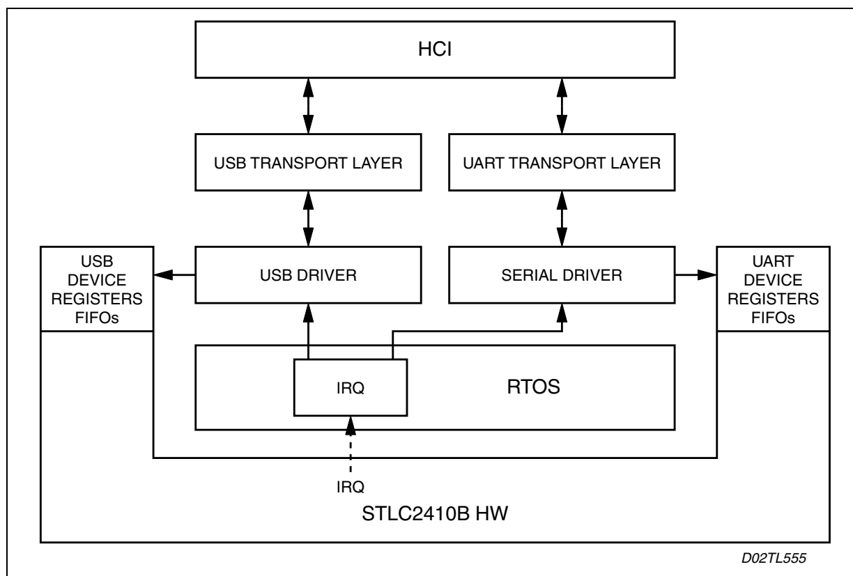
Figure 4. USB Interface
