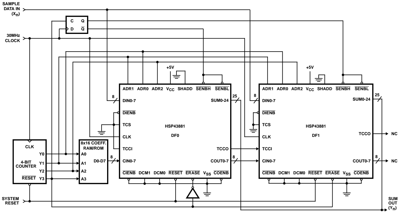
FIGURE 5. 30MHz, 16-TAP FIR FILTER CASCADE APPLICATION SCHEMATIC
