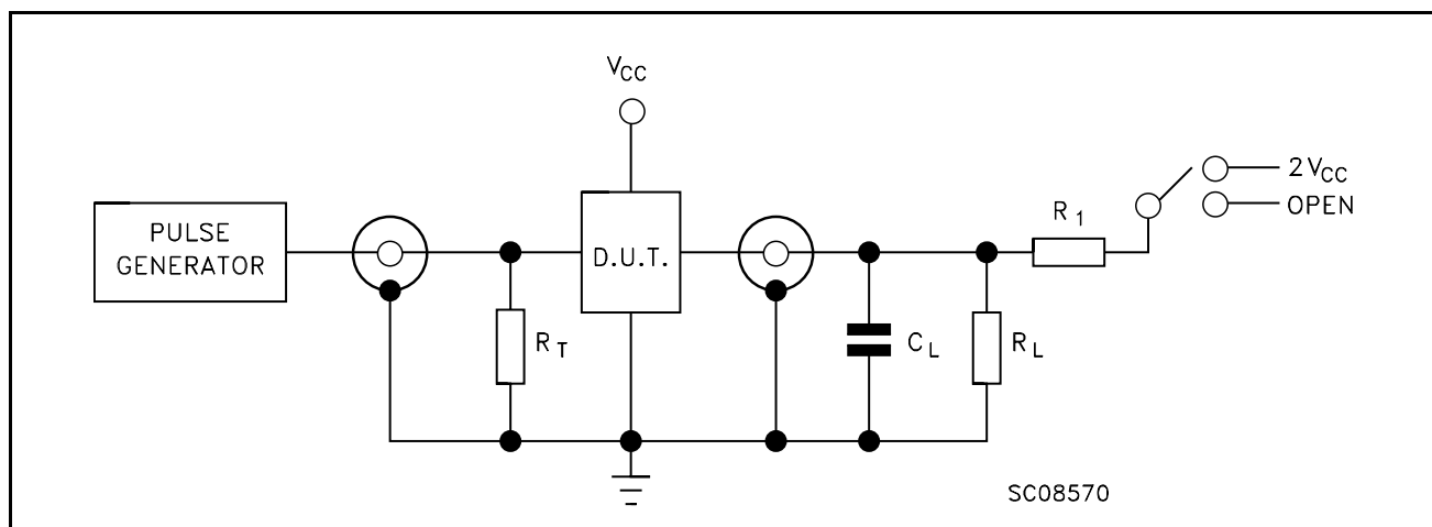
Figure 3: Test Circuit
