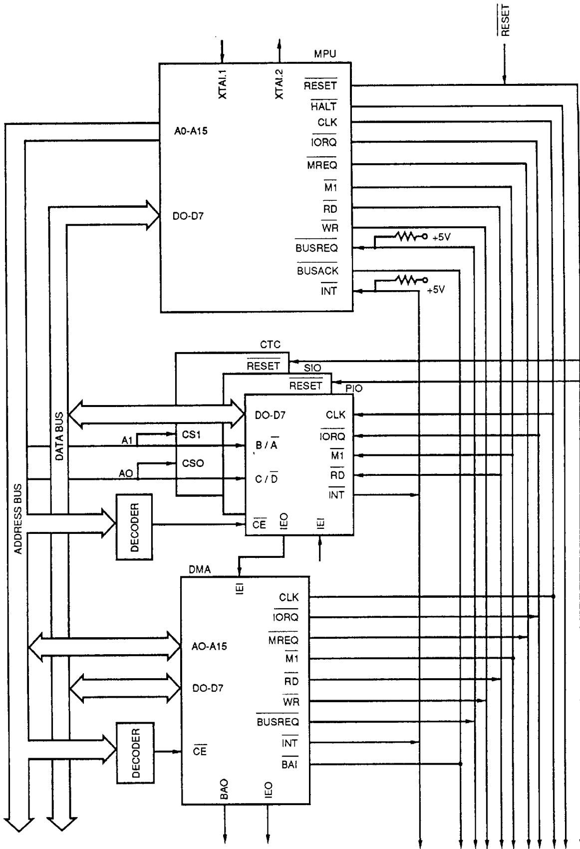
Figure 15 Example of Z80 Family Peripheral LSI
