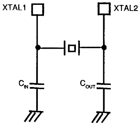
Figure 3a Example of Oscillator Connection and Constant
