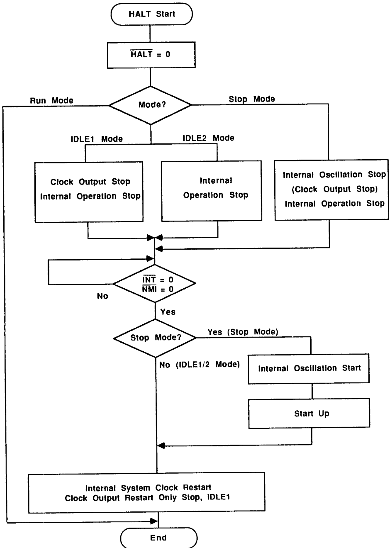
Figure 4 (b) Status Change Flowchart
