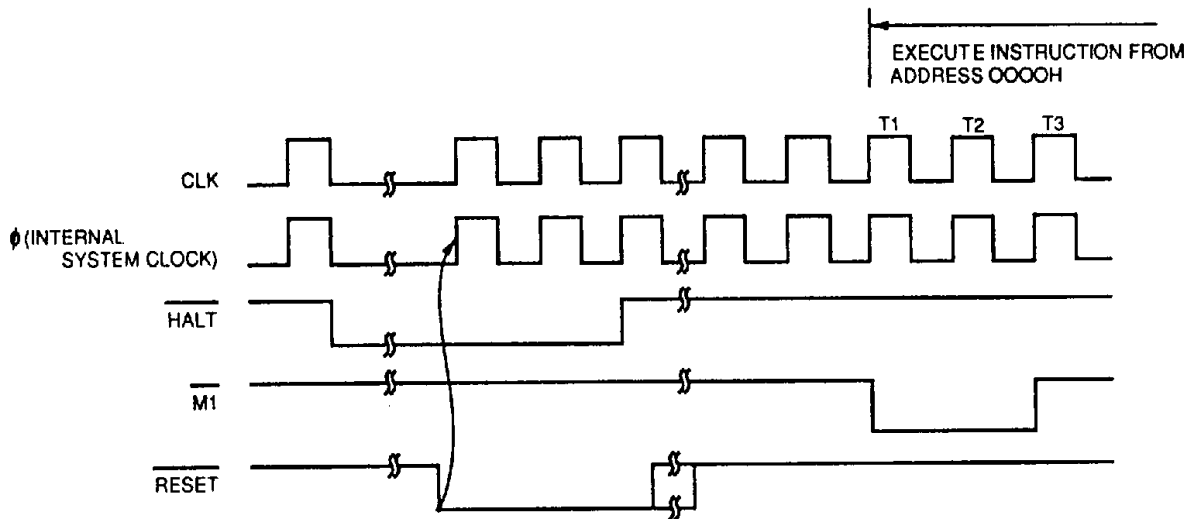
Figure 12 (a) IDLE1 Mode
