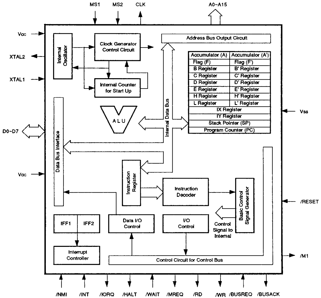
Figure 2. Block Diagram
