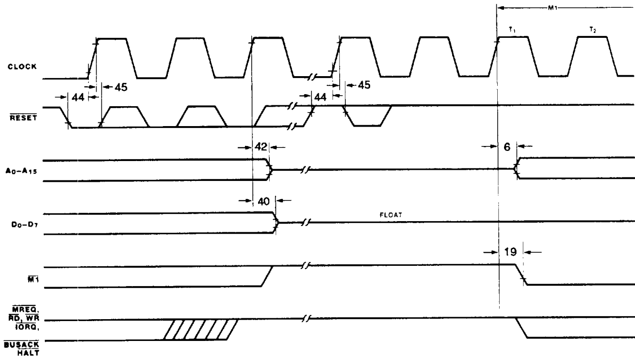
Figure 23 Reset Cycle
