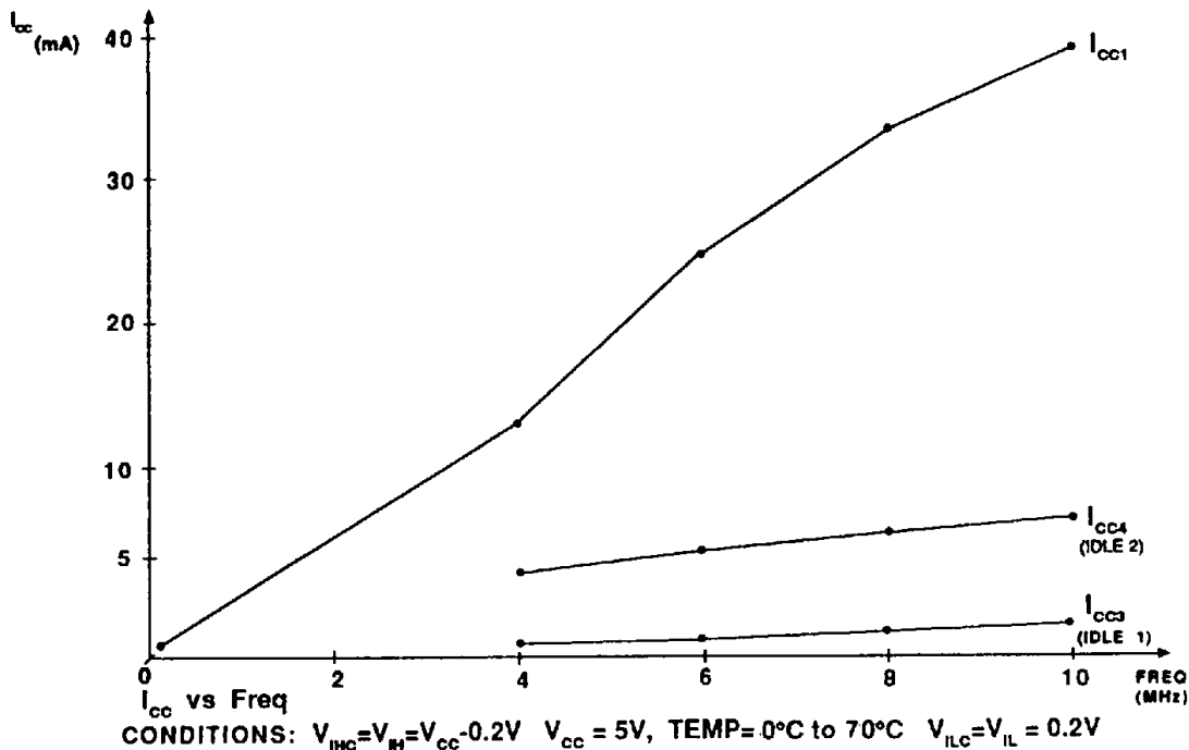
Figure 26 Z84C01 Typical I_{CC} vs Freq
