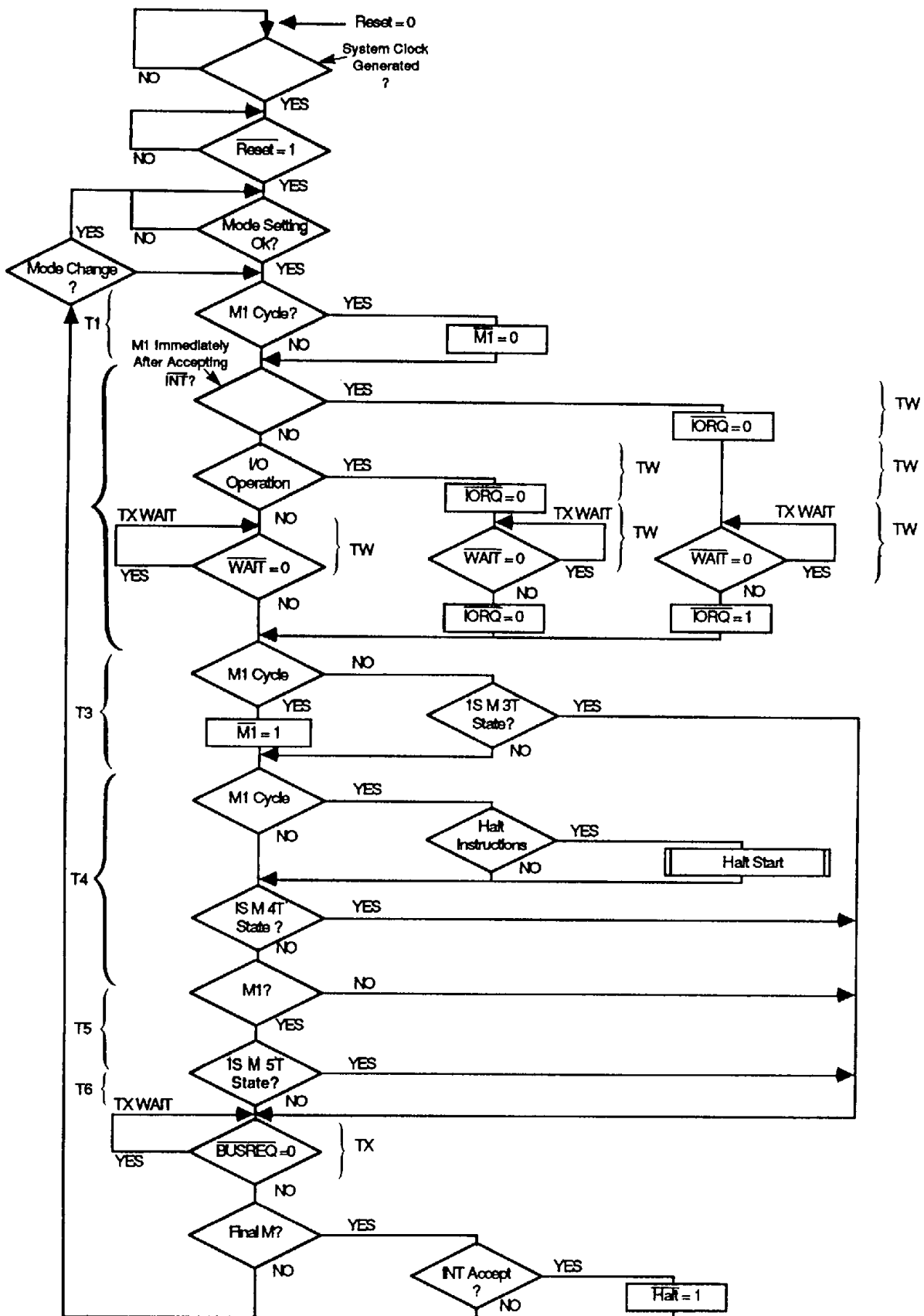
Figure 4 (a) Status Change Flowchart
