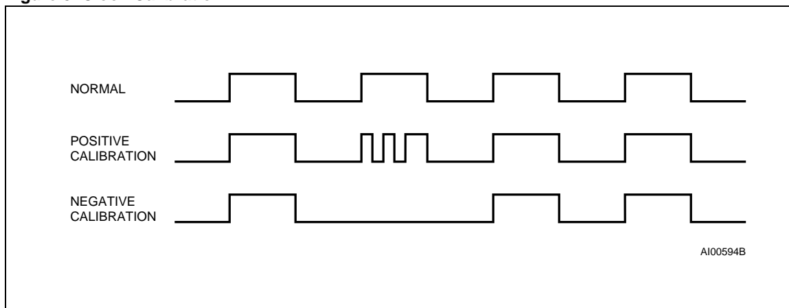
Figure 8. Clock Calibration
