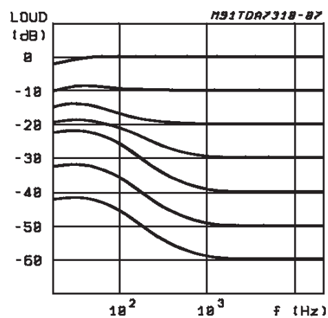
Figure 2: Loudness versus Frequency (C LOUD = 100nF)
