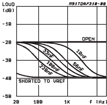
Figure 3: Loudness versus External Capacitors
