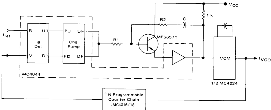
FIGURE 4 — TTL-MECL PHASE-LOCKED LOOP
