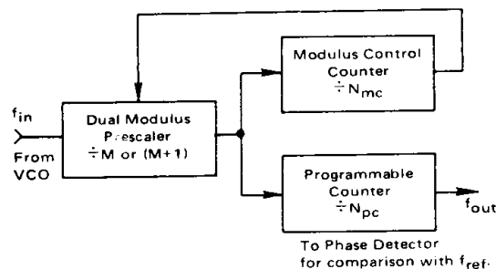
FIGURE 5 — FEEDBACK COUNTERS WITH DUAL MODULUS PRESCALER
