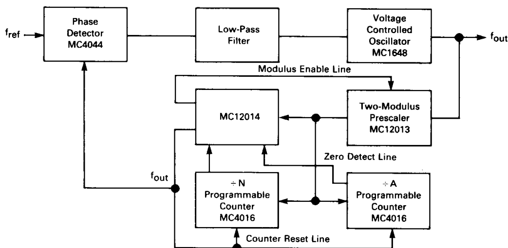
FIGURE 1 — TYPICAL FREQUENCY SYNTHESIZER APPLICATION
