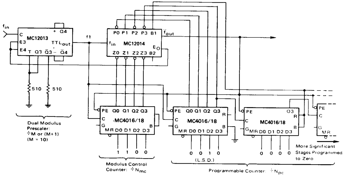
FIGURE 6 — FREQUENCY DIVISION: f_o = f_{in}/(MN_{pc} + N_{mc})
