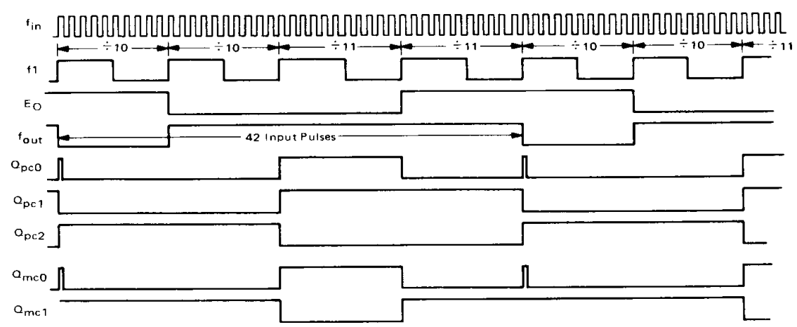
FIGURE 7b — DIVISION BY 42
