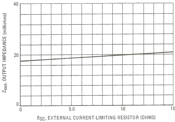
FIGURE 9 – OUTPUT IMPEDANCE versus R_{SC}
