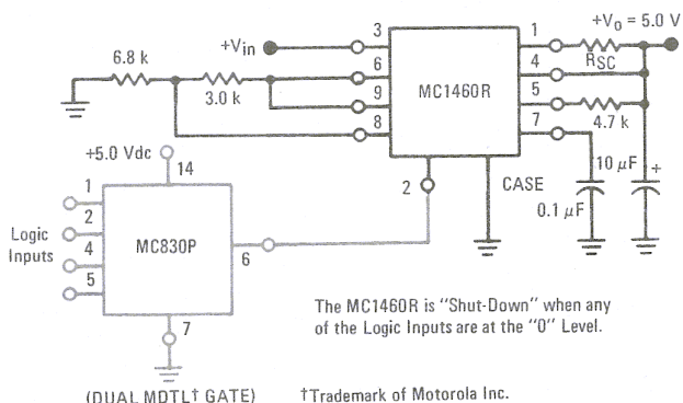
FIGURE 20 – ELECTRONIC SHUT-DOWN USING A MDTL GATE
