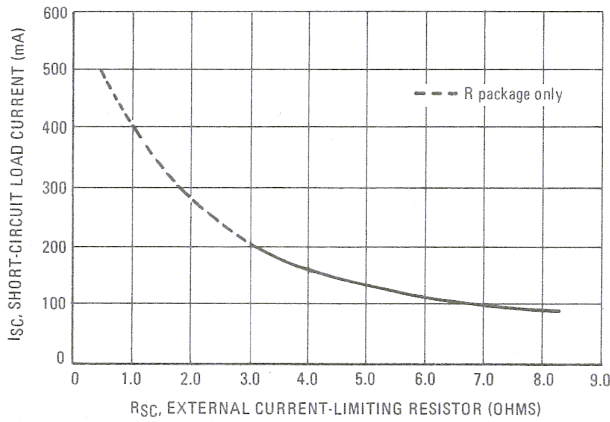
FIGURE 5 – SHORT-CIRCUIT CURRENT versus R_{SC}
