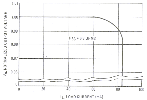
FIGURE 6 – CURRENT-LIMITING CHARACTERISTICS
