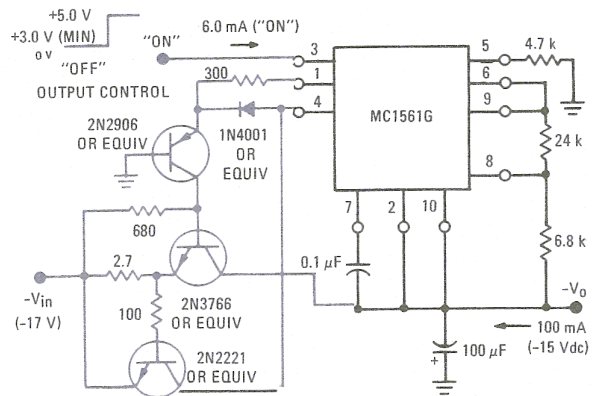
FIGURE 27 – DIGITALLY CONTROLLED 3-TERMINAL NEGATIVE REGULATOR
