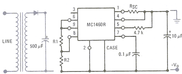
FIGURE 26 – CONNECTION FOR A NEGATIVE OUTPUT VOLTAGE
