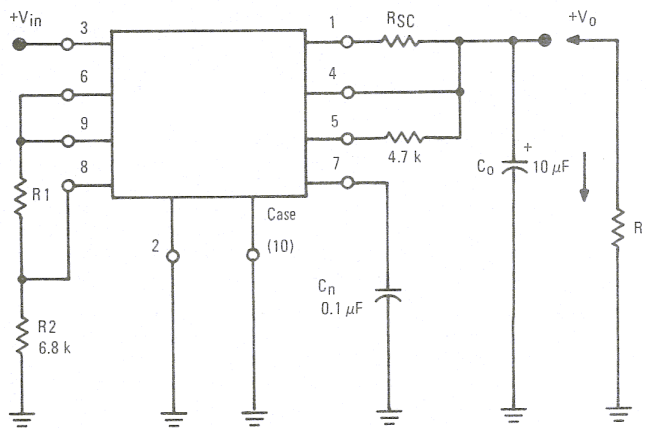
FIGURE 1 - CONNECTION FOR V_0 \geq 3.5 \text{ V}
