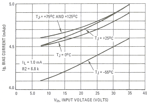
FIGURE 11 – BIAS CURRENT versus INPUT VOLTAGE
