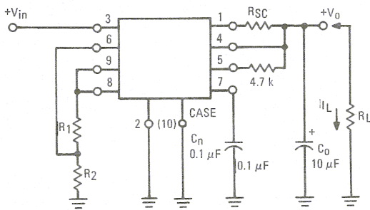
FIGURE 2 - CONNECTIONS FOR V_0 \leq +3.5 \text{ V}
