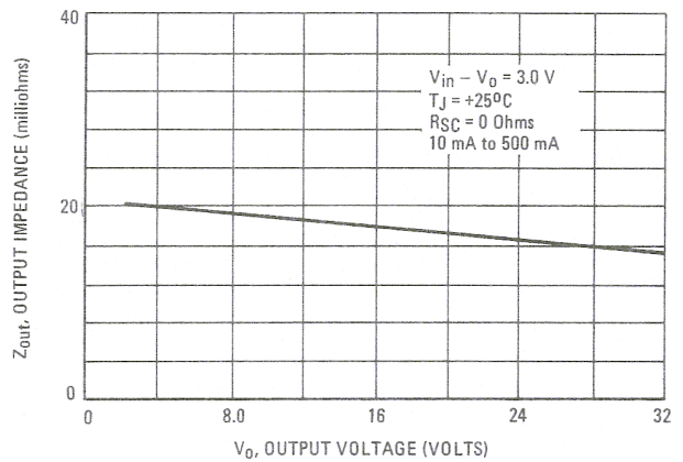
FIGURE 8 – DEPENDENCE OF OUTPUT IMPEDANCE ON OUTPUT VOLTAGE
