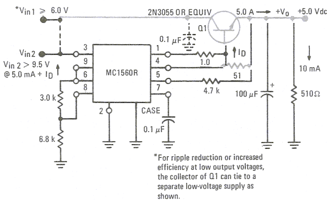
FIGURE 18 – NPN CURRENT BOOST CIRCUITS
