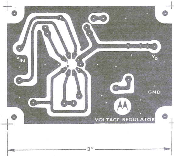
FIGURE 34 — Typical Printed Circuit Board Layout
