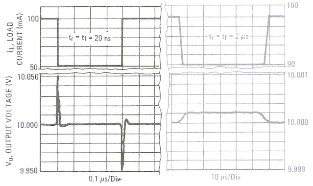
FIGURE 4 – LOAD TRANSIENT RESPONSE
