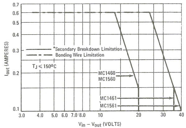
FIGURE 15b – DC SAFE OPERATING AREA ("R" PACKAGE)
