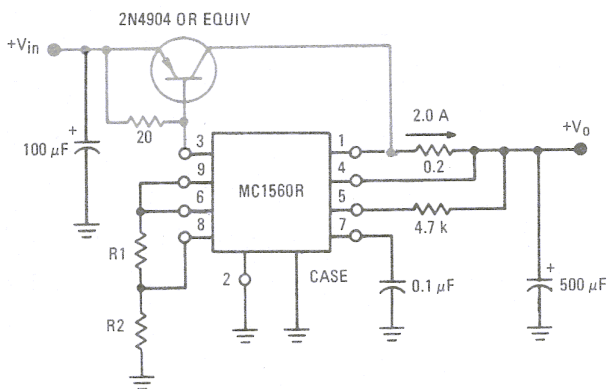
FIGURE 19 – PNP CURRENT BOOST CIRCUIT
