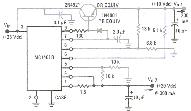
FIGURE 17 – PROVIDING TWO REGULATED OUTPUT VOLTAGES
