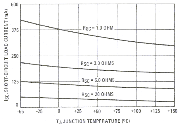
FIGURE 14 – TEMPERATURE DEPENDENCE OF SHORT-CIRCUIT LOAD CURRENT
