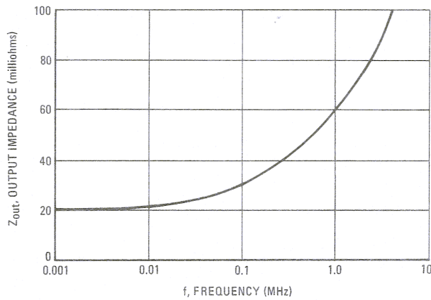
FIGURE 7 – FREQUENCY-DEPENDENCE OF OUTPUT IMPEDANCE
