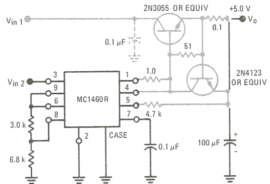
FIGURE 18 – NPN CURRENT BOOST CIRCUITS
