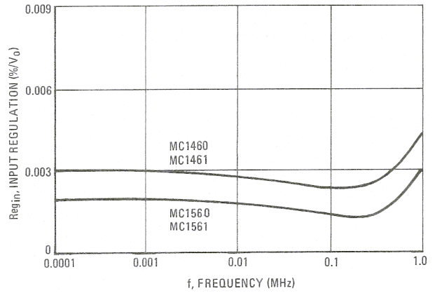
FIGURE 10 – FREQUENCY-DEPENDENCE OF INPUT REGULATION
