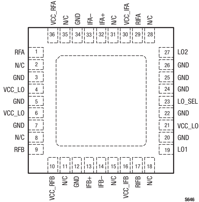
Figure 2. SKY73087-11 Pinout – 36-Pin MCM (Top View)
