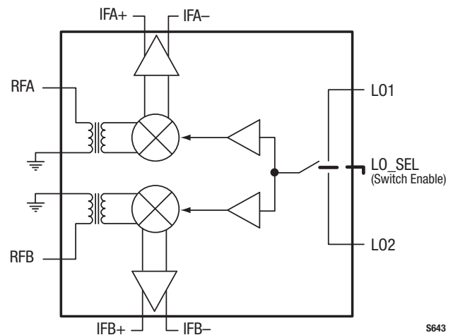
Figure 1. SKY73087-11 Block Diagram
