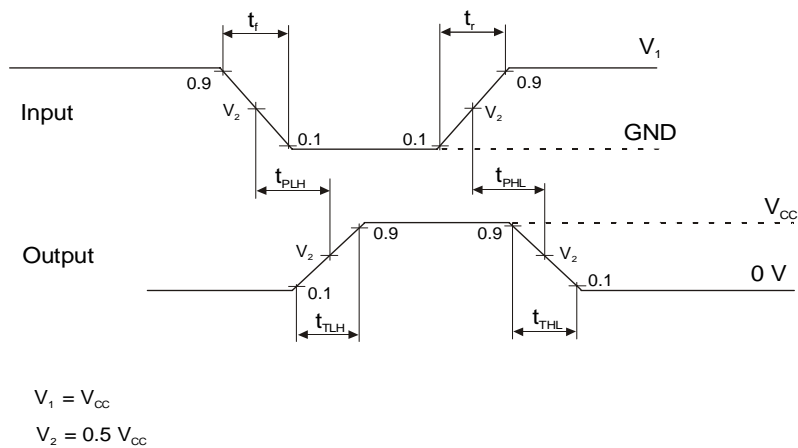
Figure 1. Switching Waveforms
