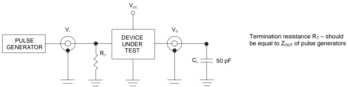
Figure 2. Test Circuit
