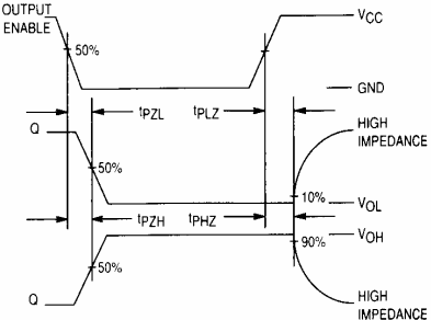
Figure 2. Switching Waveforms
