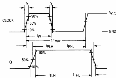
Figure 1. Switching Waveforms
