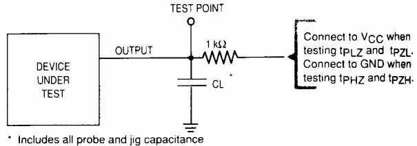
Figure 5. Test Circuit
