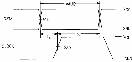
Figure 3. Switching Waveforms
