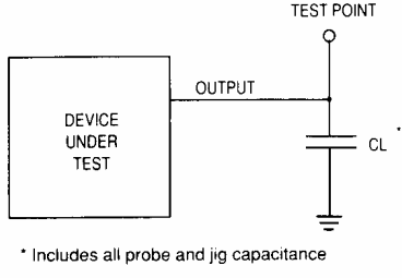
Figure 4. Test Circuit
