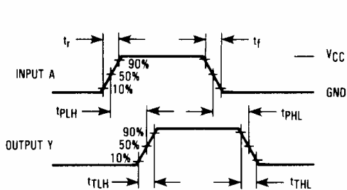
Figure 1. Switching Waveforms
