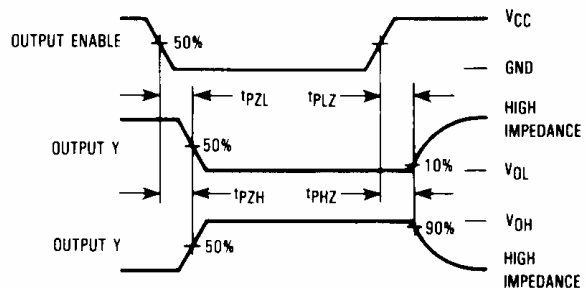
Figure 2. Switching Waveforms
