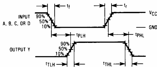
Figure 1. Switching Waveforms
