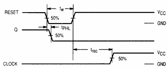
Figure 2. Switching Waveforms
