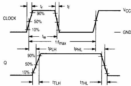
Figure 1. Switching Waveforms
