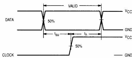
Figure 3. Switching Waveforms
